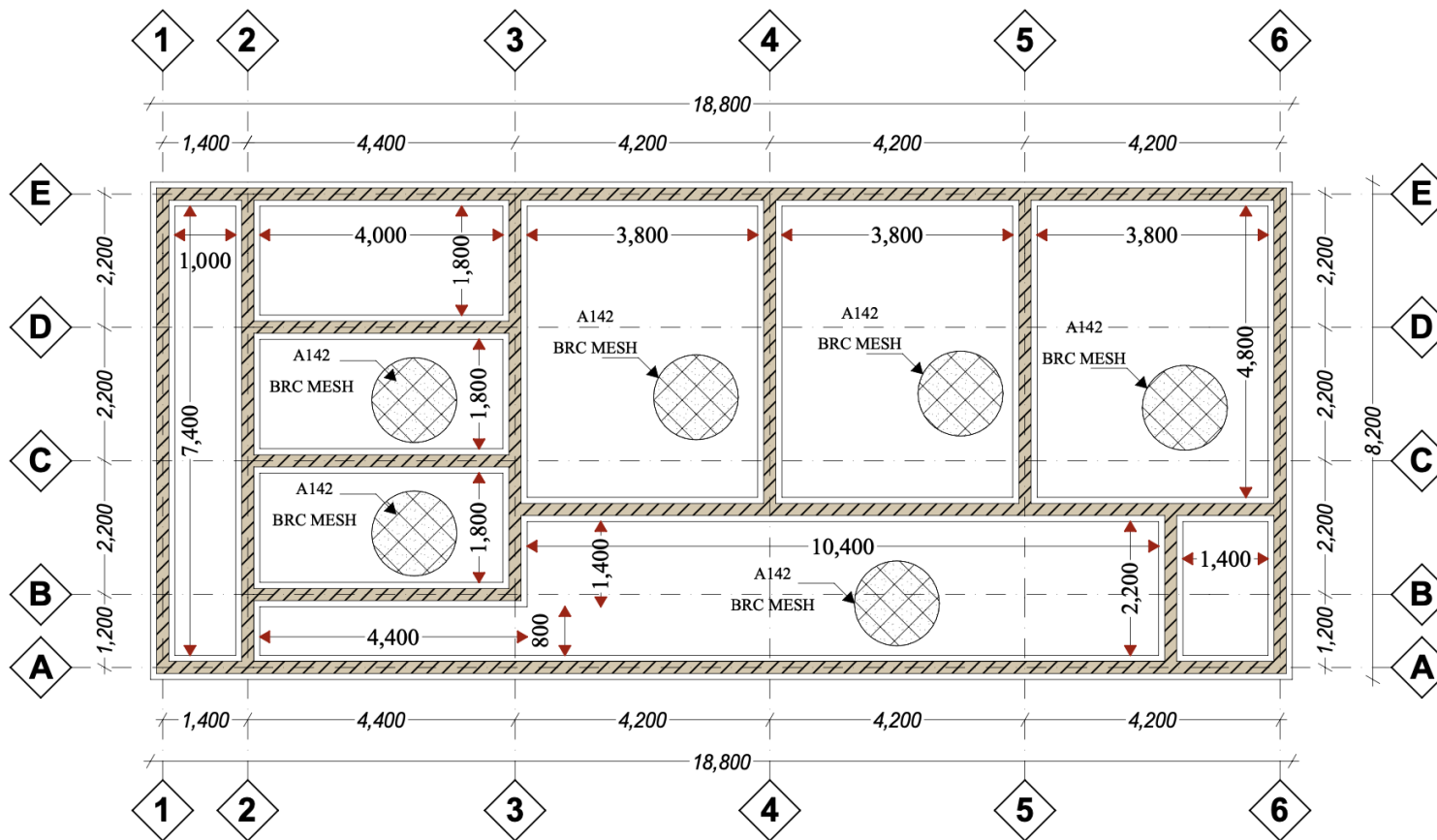
FOUNDATION LAYOUT
