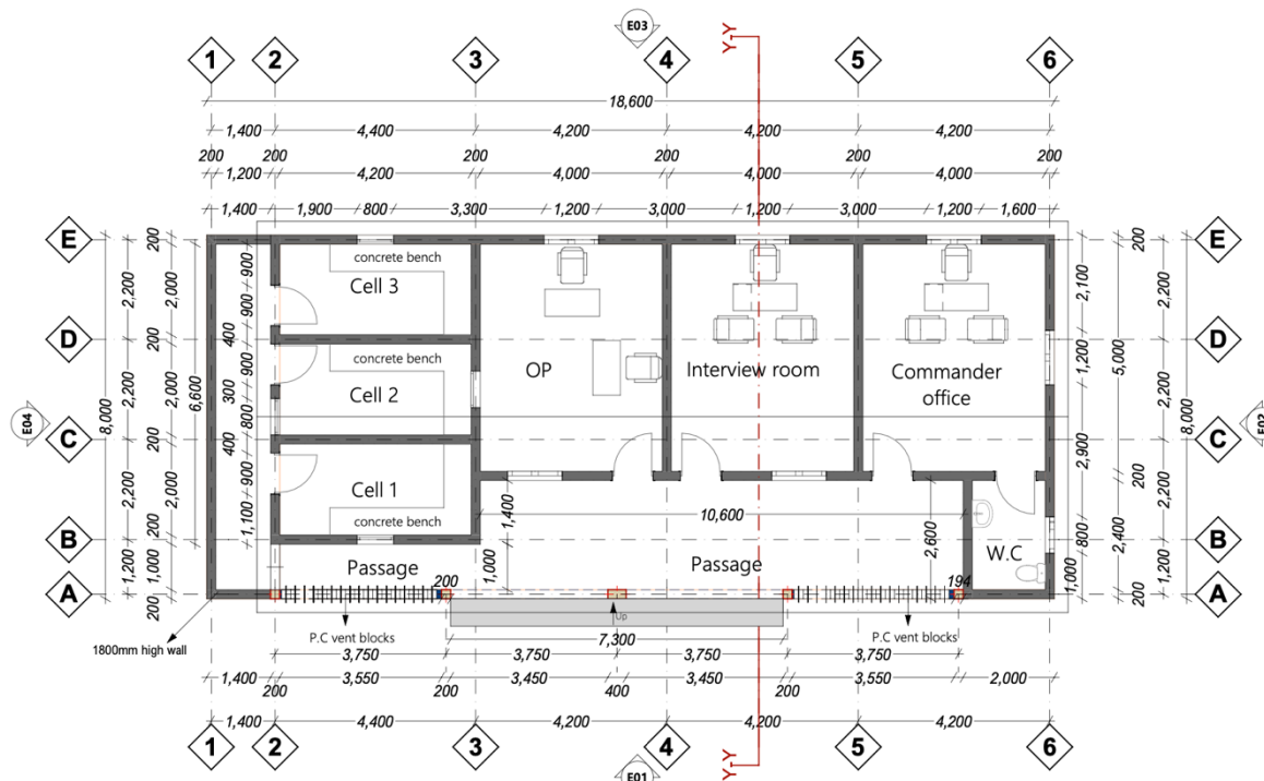
FLOOR LAYOUT
