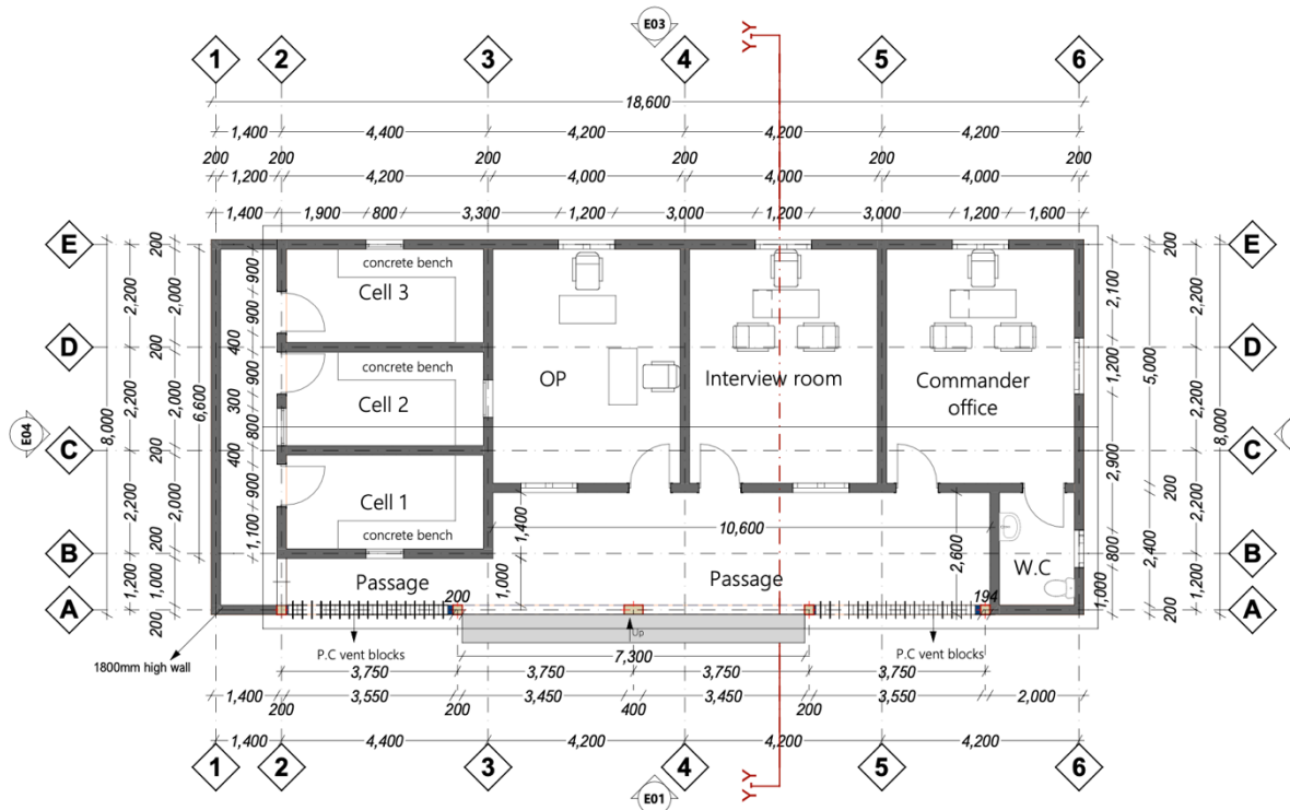
FLOOR LAYOUT
